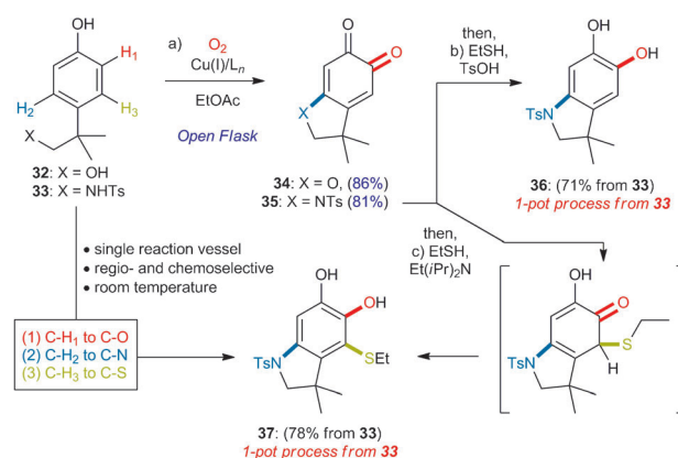
Scheme 3. Cross-aerobic coupling. Reagents and conditions: a) Synthesis of 34 and 35 : 3 (4 mol%), DBED (5 mol%), EtOAc (0.5 M), open flask. Synthesis of 36 from 33 : 3 (4 mol%), DBED (5 mol%), CH 2 Cl 2 (0.1 M), O 2 (1 atm); then EtSH (4 equiv), para -toluenesulfonic acid (1 equiv). Synthesis of 37 : 3 (4 mol%), DBED (5 mol%), CH 2 Cl 2 (0.1 M), O 2 (1 atm); then EtSH (4 equiv), DBED (1 equiv).
